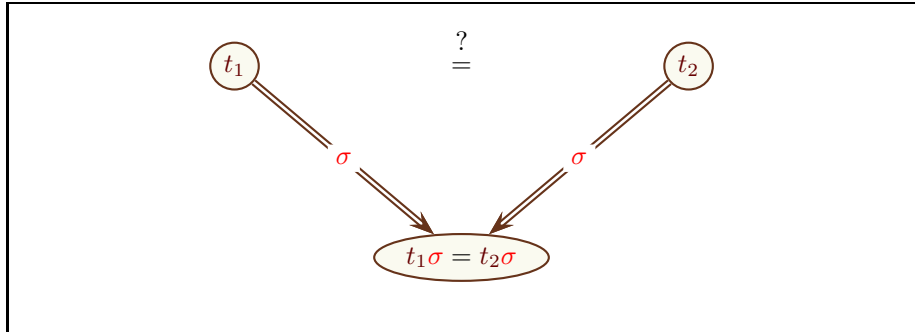
Figure 2: \mathcal{FOT} unification as a constraint
