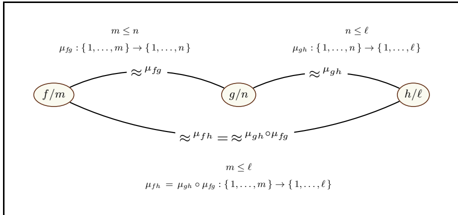
Figure 10: Compositional Consistency Condition for Non-Aligned \mathcal{FOT} Argument Alignment Mappings
