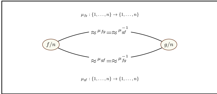
Figure 9: Invertibility Consistency Condition for Equal-Arity \mathcal{FOT} Argument Alignment Mappings
