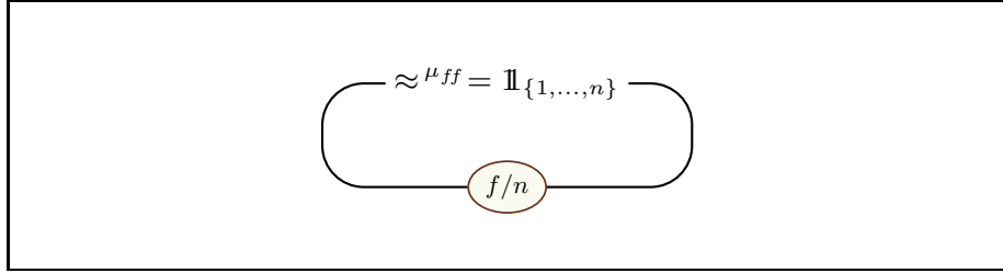
Figure 8: Identity Consistency Condition for \mathcal{FOT} Argument Alignment Mapping
