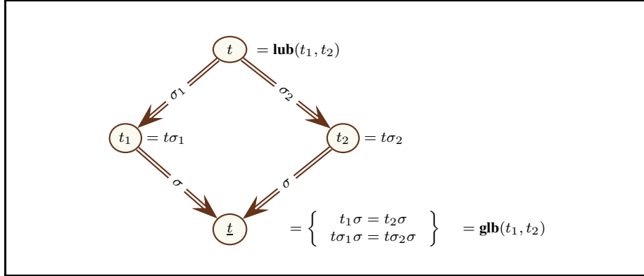
Figure 1: Subsumption lattice operations
