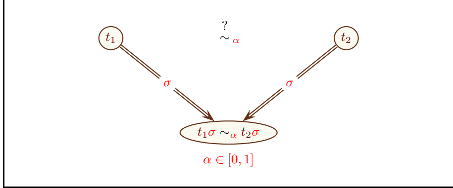
Figure 6: Fuzzy unification as a constraint
