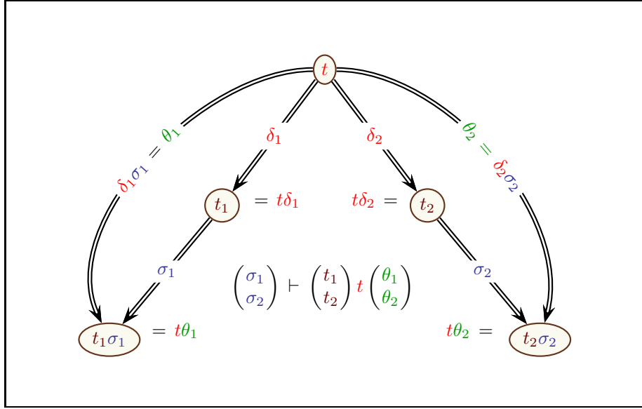
Figure 4: \mathcal{FOT} generalization judgment validity as a constraint
