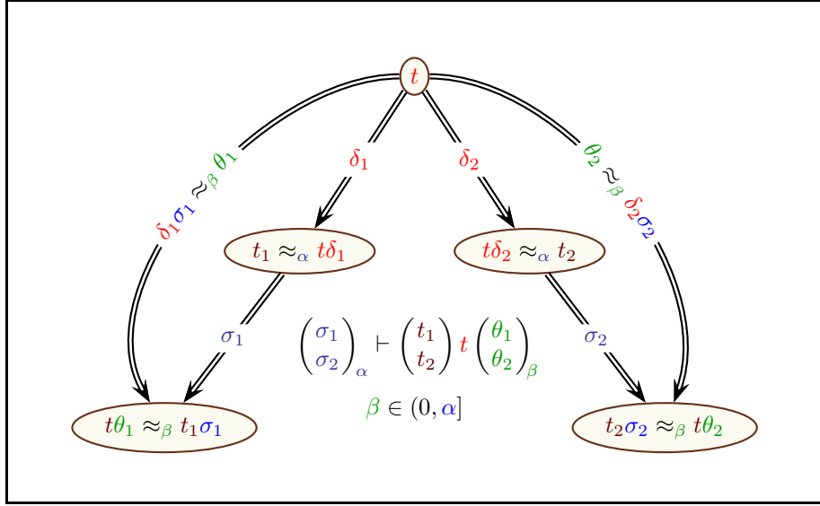
Figure 12: Fuzzy generalization judgment validity as a constraint
